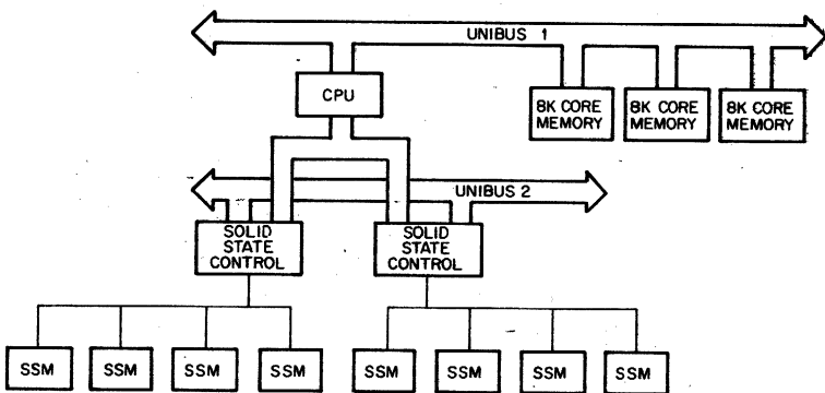
Figure 2-7 Memory Configuration
