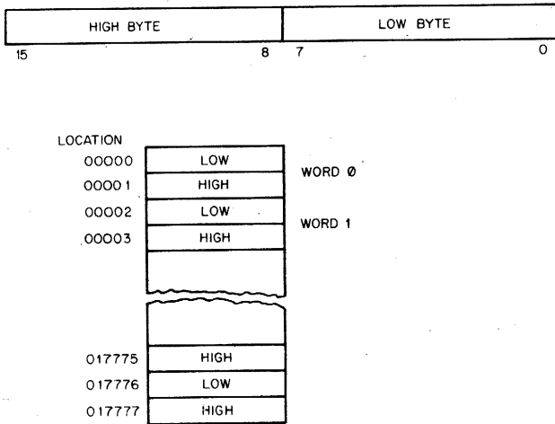
Figure 2-9 Memory Organization
