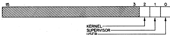
Figure 6-10: Format of Status Register #3 (SR3)
