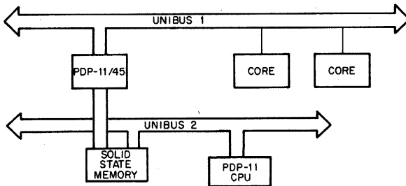
Figure 2-8 Multiprocessor Use of the Second UNIBUS
