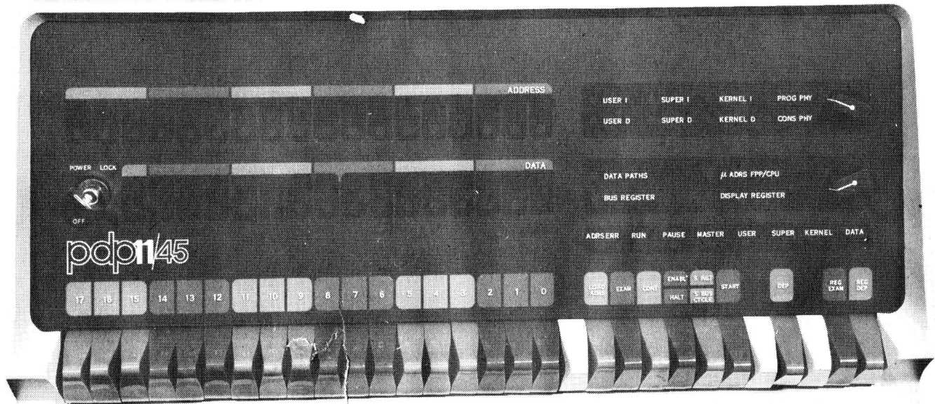
Figure 8-1 System Operator's Console
