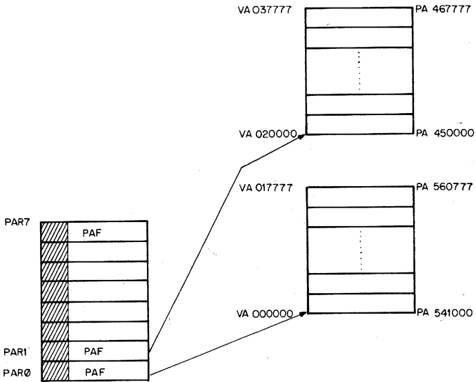
Figure 6-12: Non-Consecutive Memory Pages
